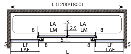
PROFILI A TERRA FLOOR PROFILES - BODENPROFILE ▶ 106
