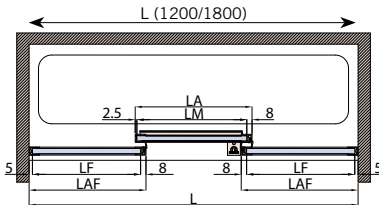
PROFILI A TERRA FLOOR PROFILES - BODENPROFILE
