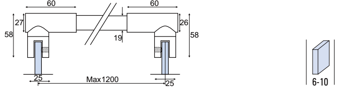
B-166 €► BX.330 • Terminali per barra. • Articulated glass to wall bar. • Drehbar Messing geschmiedet. CR - NS
